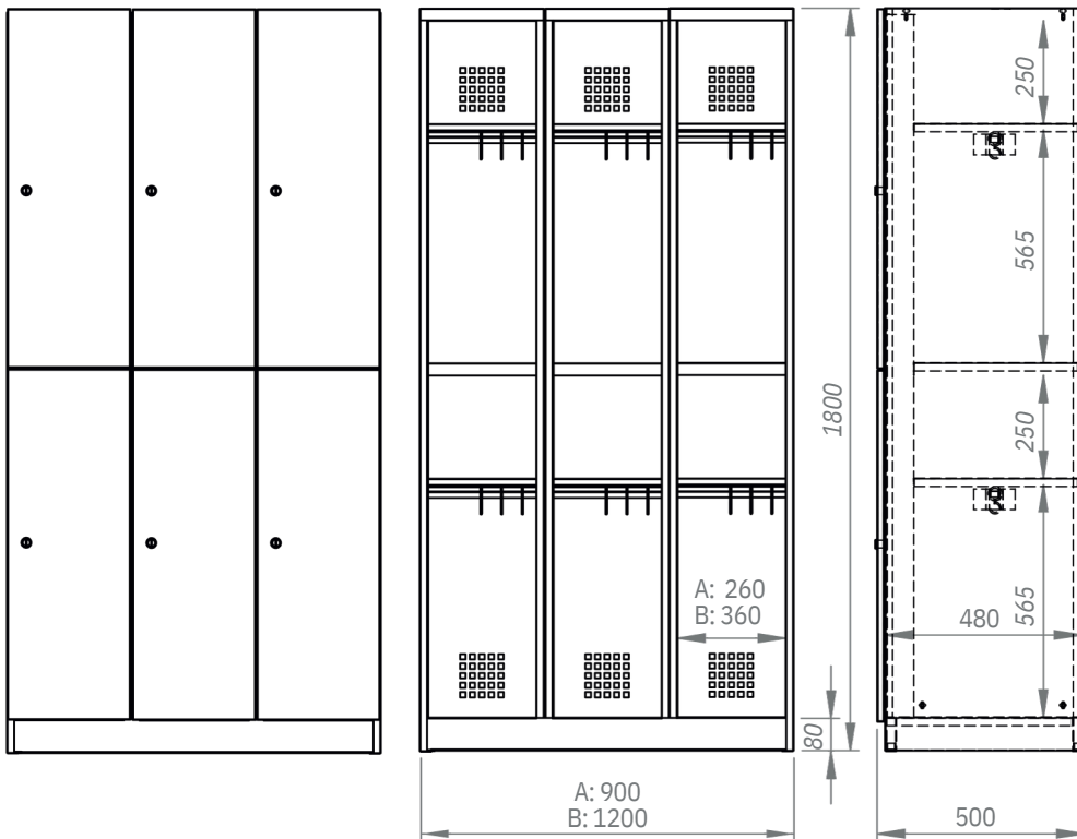
AQUARIUS SG3302P (A) AQUARIUS SG3402P (B)
