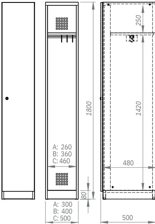
AQUARIUS SG1301P (A) AQUARIUS SG1401P (B) AQUARIUS SG1501P (C)
