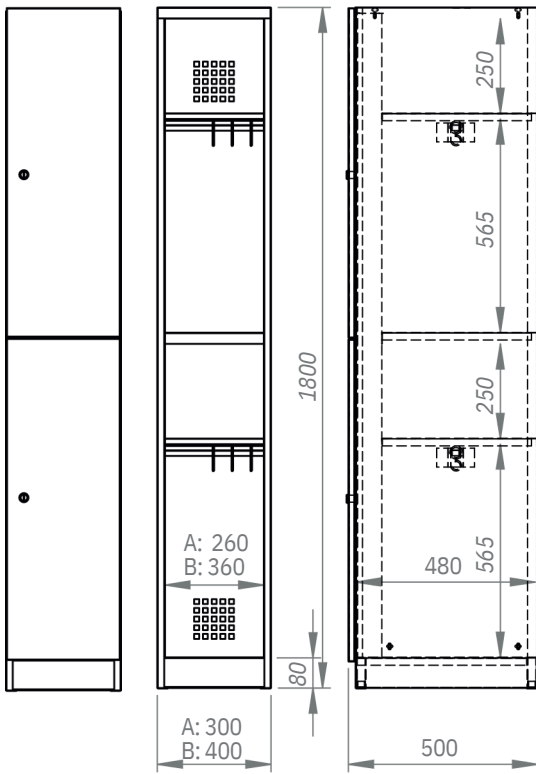
AQUARIUS SG1302P (A) AQUARIUS SG1402P (B)
