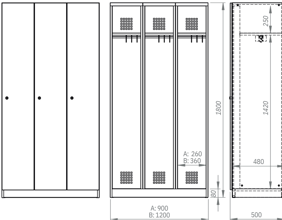
AQUARIUS SG3301P (A) AQUARIUS SG3401P (B)
