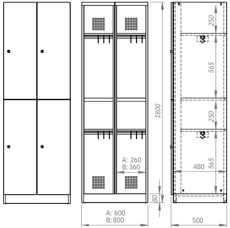
AQUARIUS SG2302P (A) AQUARIUS SG2402P (B)
